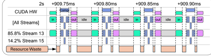
Fig. 1: Gaps between operations in Nsight profiler
