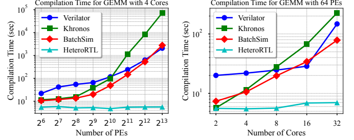
Fig. 3: Compilation time of GEMM accelerators across different RTL simulators under varying Rocket core and PE configurations.
