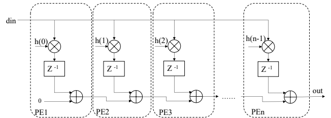
Fig. 1. Hardware structure of pulsation FIR filter
